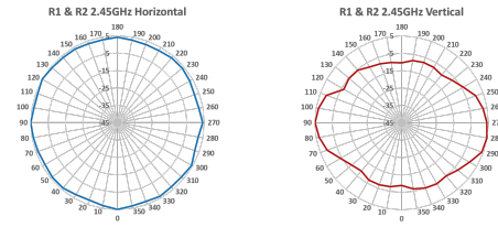
FAP-233G Radio 1&amp;2 antenna plots
